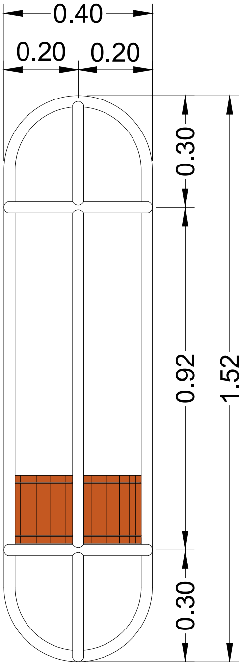
LATERAL
